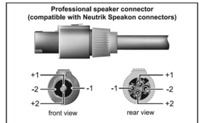
Fig. 4.1: Neutrik Speakon-compatible connectors
